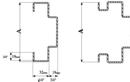
Construction frame
